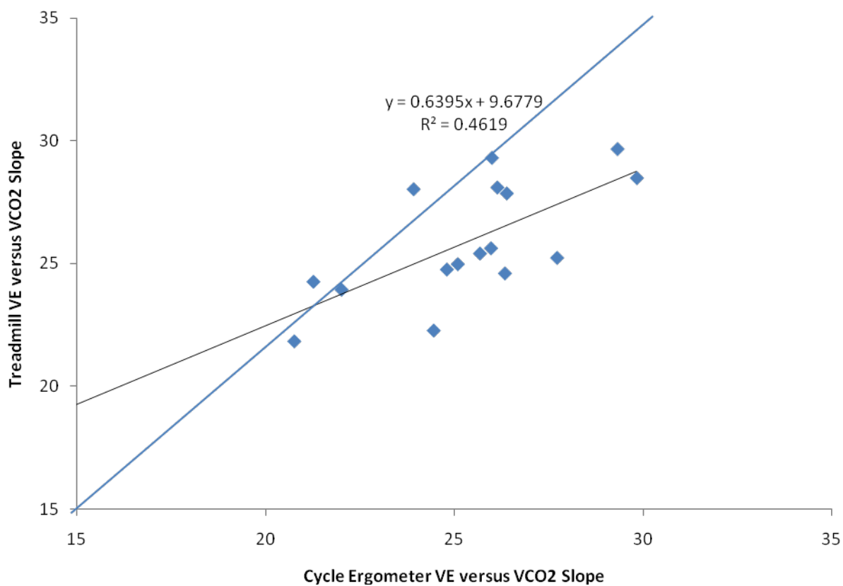
Figure 2. Scatter diagram of the overall V_E/V_{CO_2} slope for the treadmill and cycle ergometer
